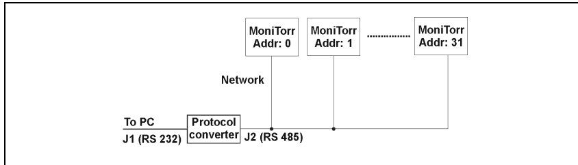
Figure 25 Network connection
