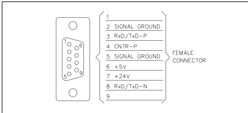
Figure 40 ProfiBus connector
